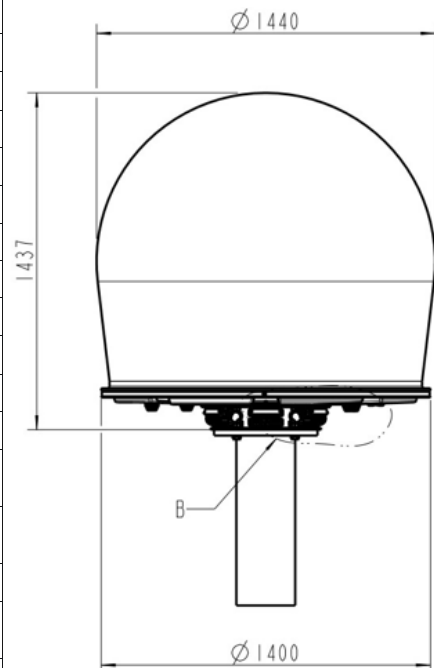
Figure 1, Radom Size in mm (indicative maximum figures)
